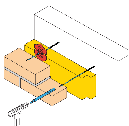
10. UNI-CB-spouwanker
