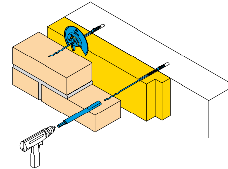
8. UNI-plug
