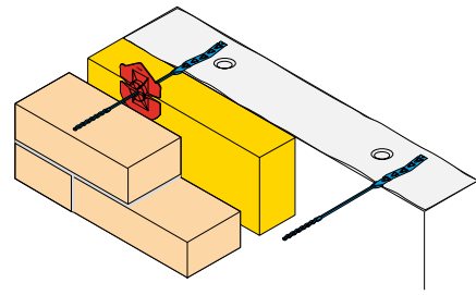
1. Prikspouwanker
