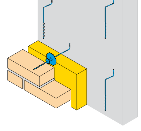
11. UNI-prefab-spouwanker
