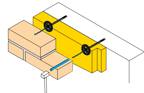
8. UNI-plug
