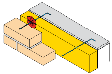
4. UNI-L-spouwanker
